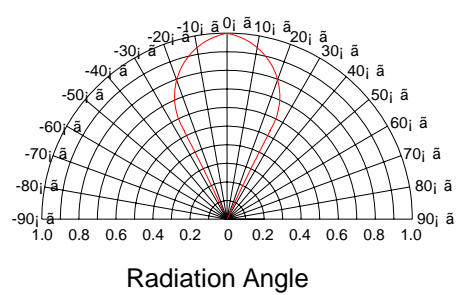
Radiation Characteristics
